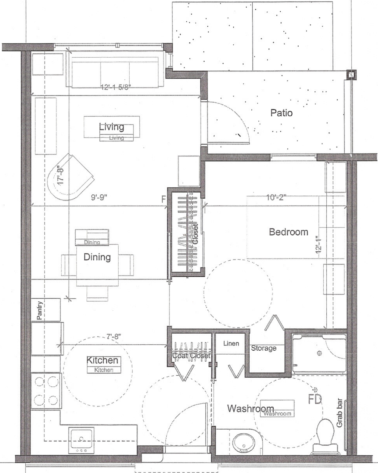
Main Floor Type A
